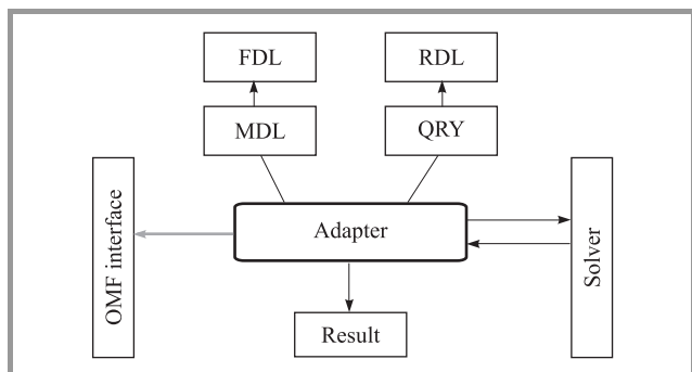
Fig. 2. An input/output view of Telemaco
