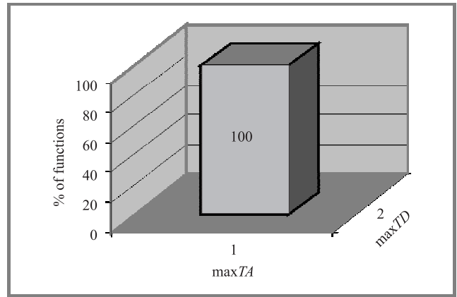
Fig. 1. Distribution for permutations and arbitrary functions ( n = 1, m = 1 ).
