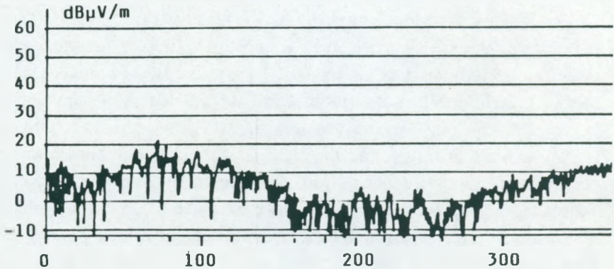
Fig. 1. Field strength variations in a small area
